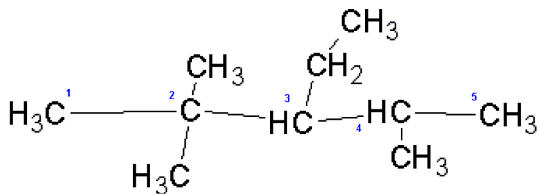
3-ethyl-2,2,4-trimethylpentane
