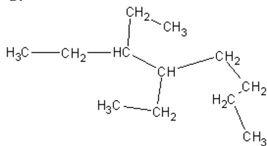
3,4-diethyloctane
