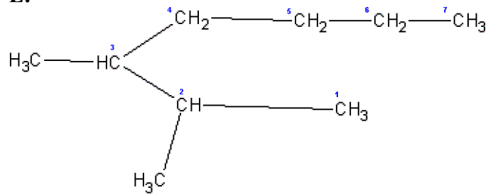
2,3-dimethylheptane
