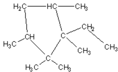
1-ethyl-1,2,2,3,5-pentamethylcyclopentane 11
