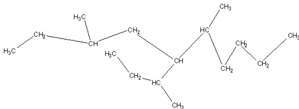
5-(butan-2-yl)-3,6-dimethyldecane
