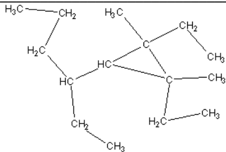
1,2-diethyl-3-(hexan-3-yl)-1,2-dimethylcyclopropane 12
