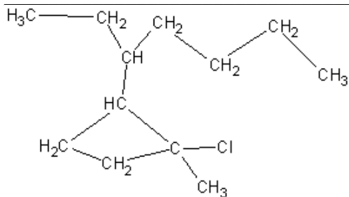
1-chloro-2-(heptan-3-yl)-1-methylcyclobutane 14
